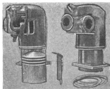
Cylinders Have Electrically Deposited Water Jackets.
